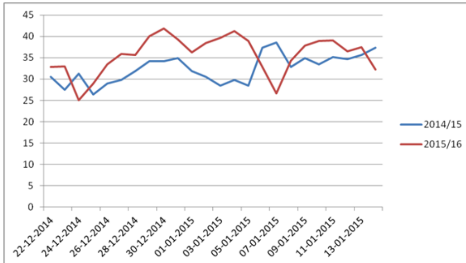
Maximum temperatures for 2014/15 and 2015/16 for Ceres.
